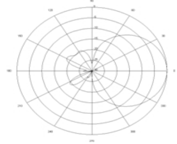
RF Patterns Horizontal Cut, typ.
