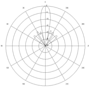
RF Patterns Vertical Cut, typ.
